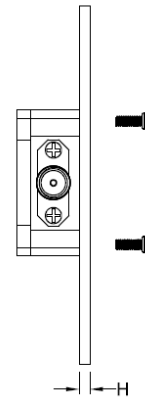
Lateral View Fig 3
