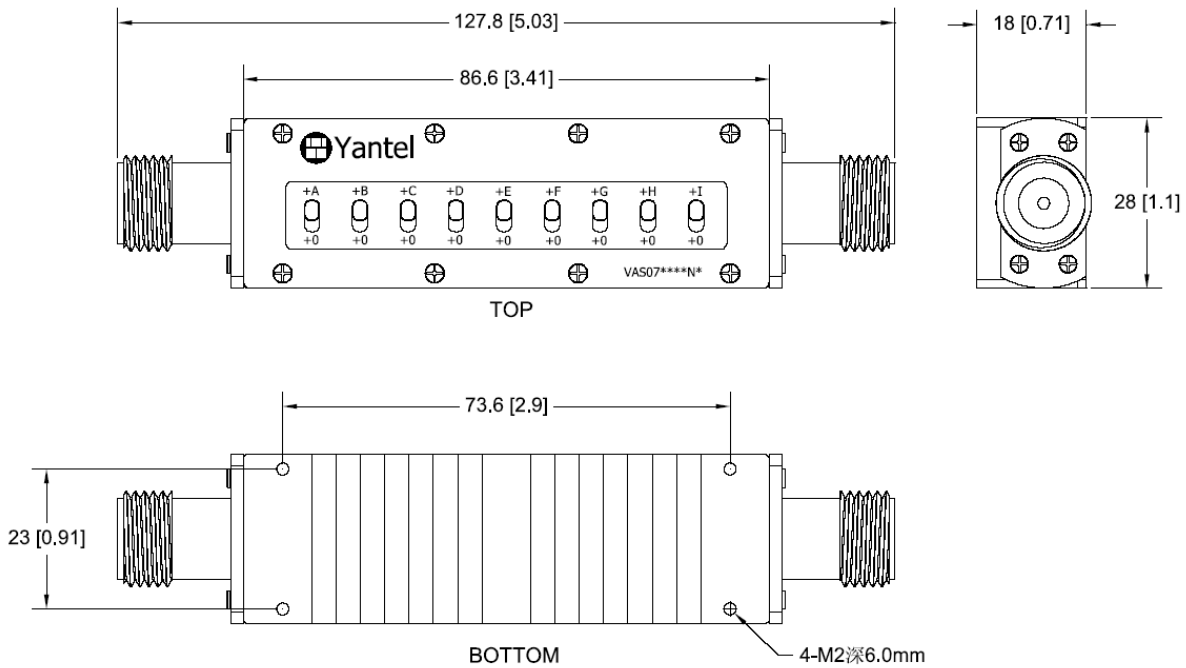
Package type: N51
