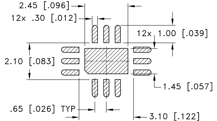
SUGGESTED LAYOUT FOR PCB LAND PATTERN (TOL ±.002)
