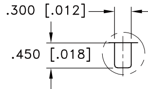
DETAIL "A" SCALE 16:1 12 PLCS
